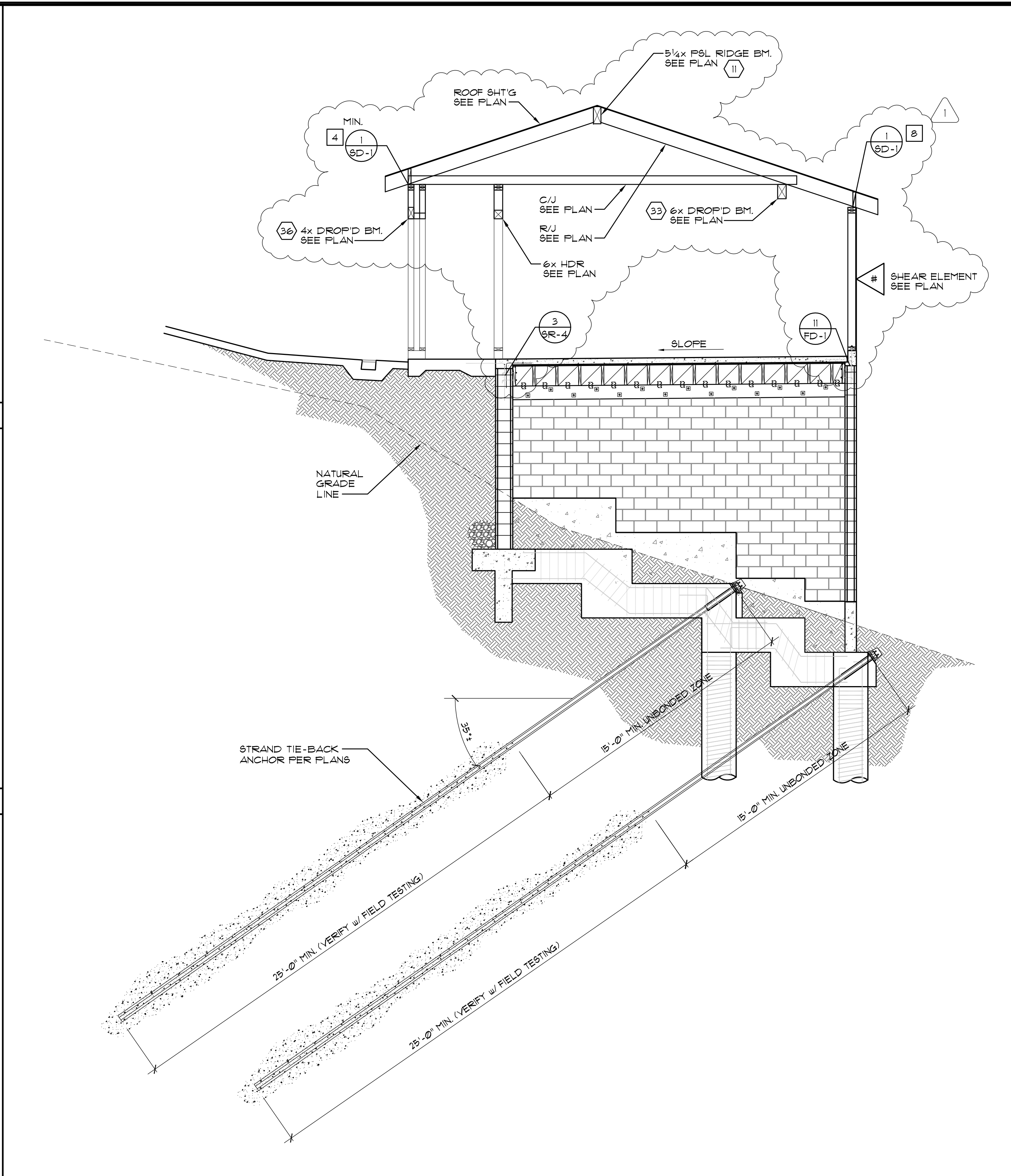
STRUCTURAL SECTION
