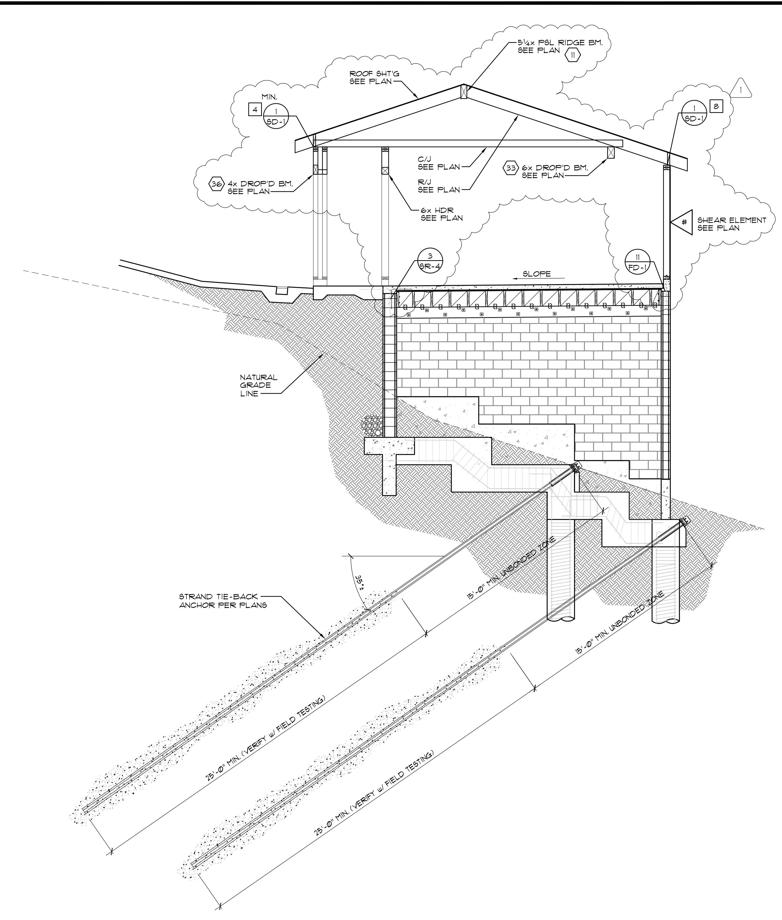
STRUCTURAL SECTION
