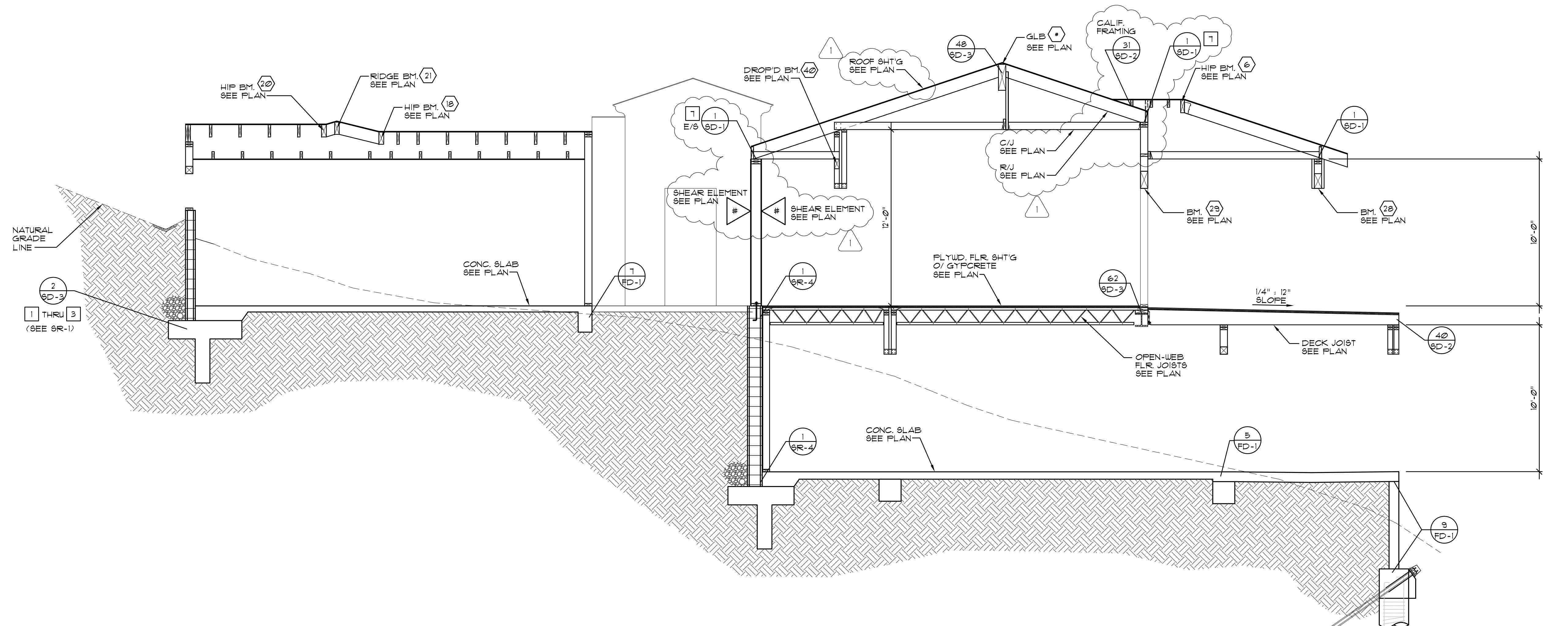
STRUCTURAL SECTION
