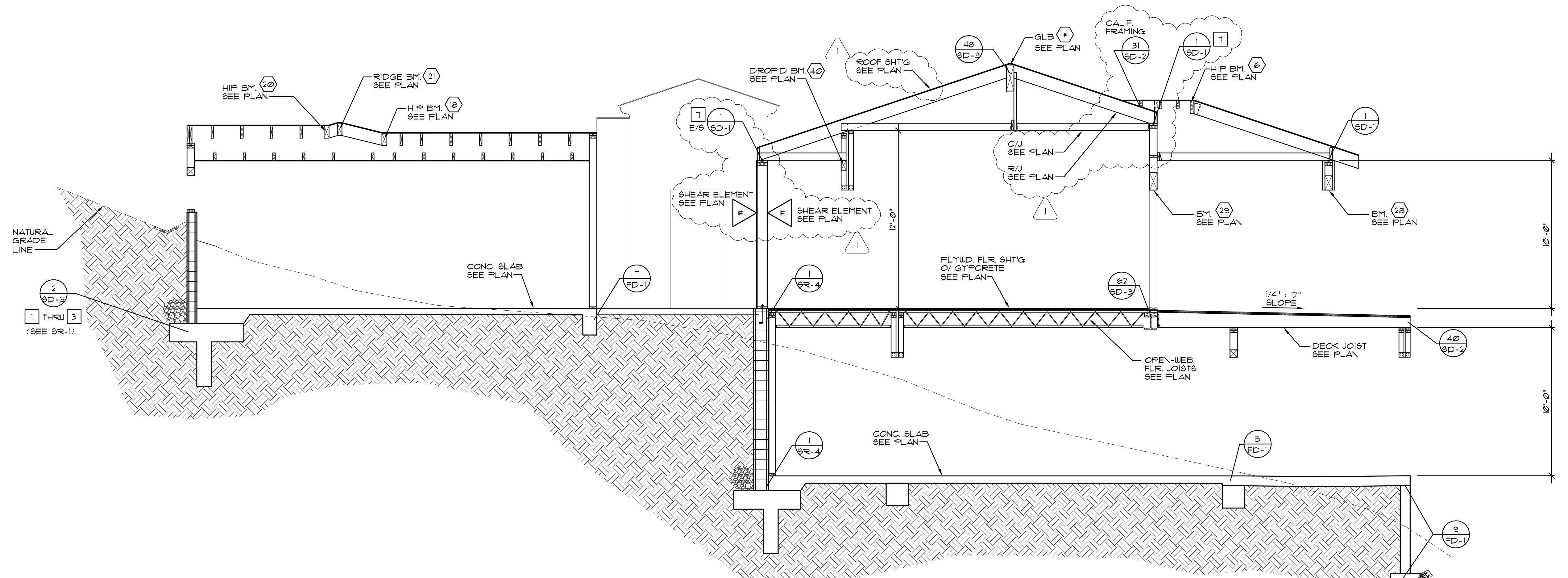
STRUCTURAL SECTION
