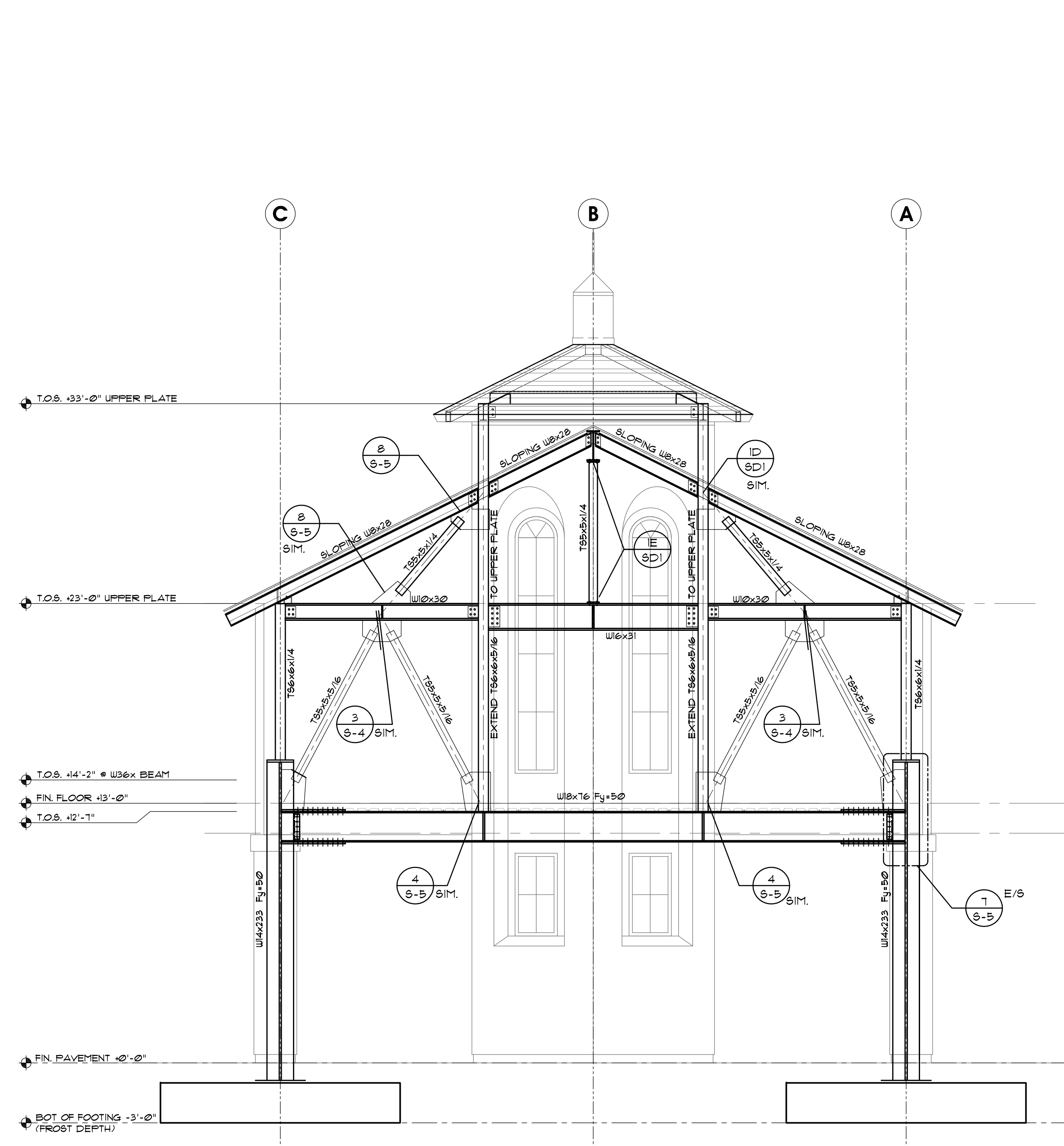
B. FRAME ELEVATION @ GRID 2 SCALE 1/4" = 1'-0"
