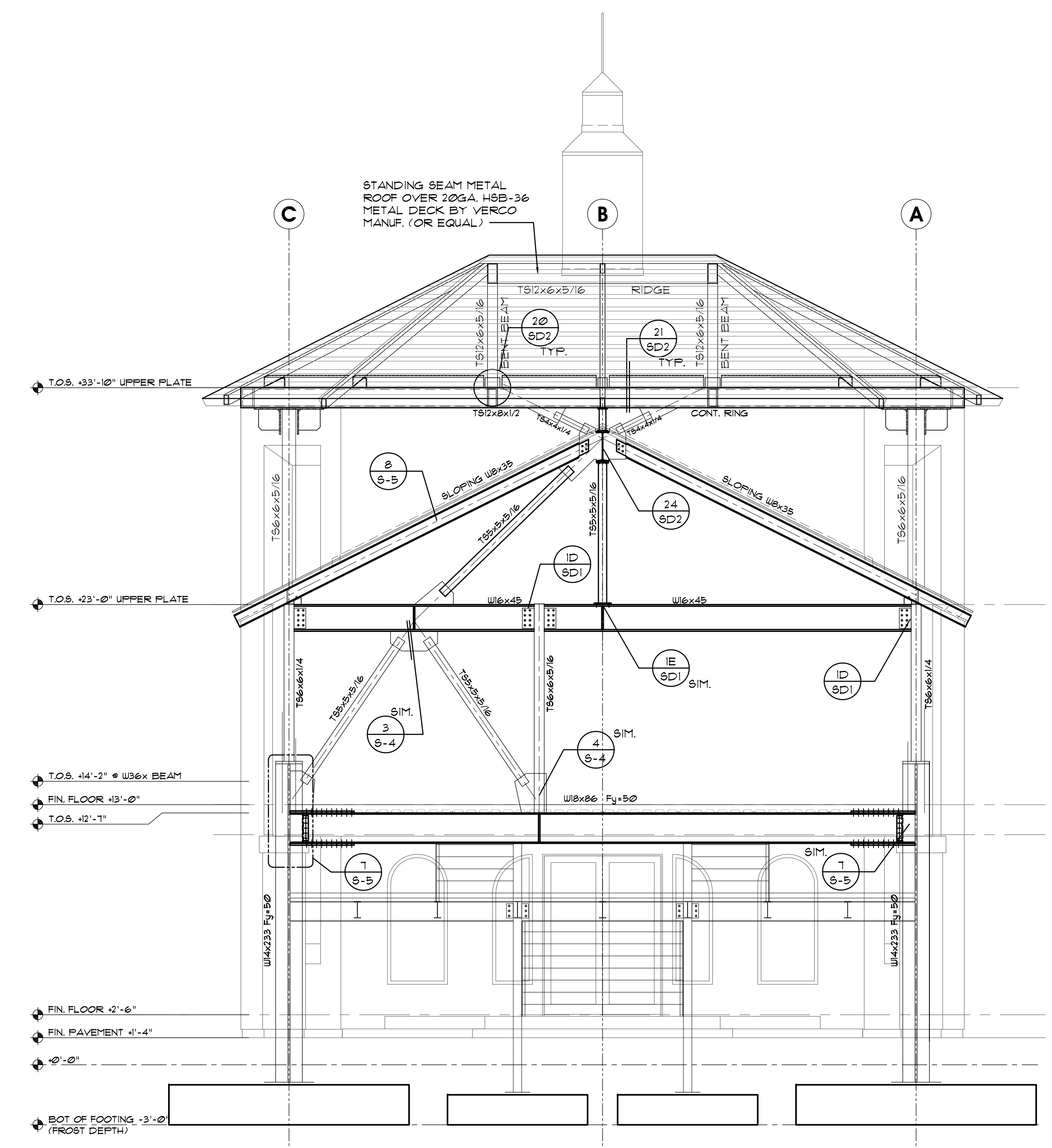
C. FRAME ELEVATION @ GRID 3 SCALE 1/4" = 1'-0"
